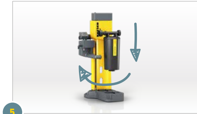
5 The new cartridges are inserted in reverse sequence accordingly. The screw connection clamping nuts are tightened – refer to step 2.
