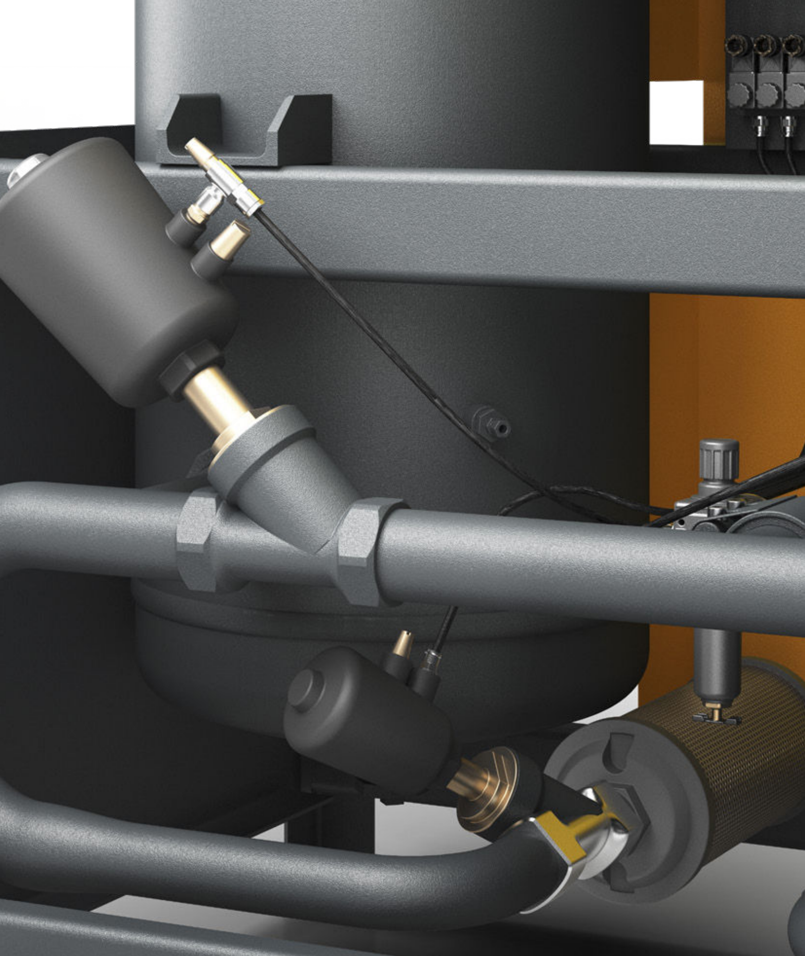
Image: i.DC 140 with high-quality oil/water separators at the compressed air inlet and regeneration air outlet
