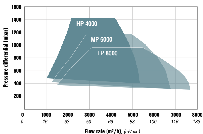
Image: Characteristic map for 150 kW series
