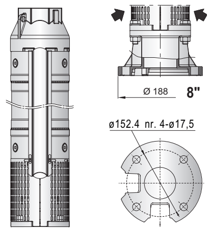
Reinforced with special collar from 6SDX(L) 46/27
